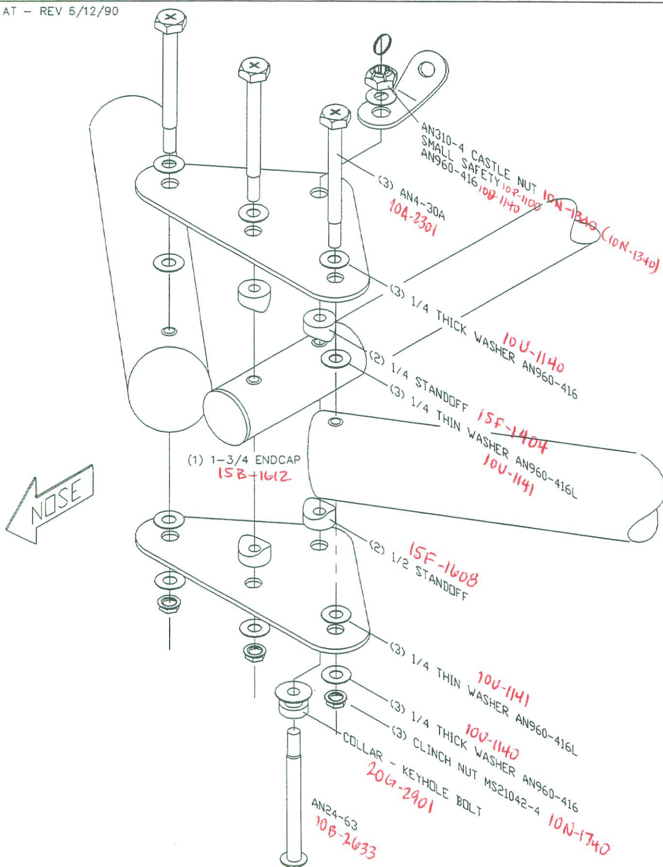
HP AT NOSEPLATE ASSEMBLY
